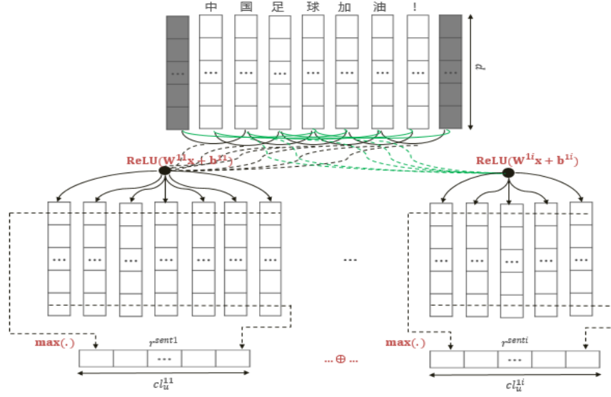
图2 通过基于不同窗口大小的卷积方法利用多个不同大小的卷积核抽取句子级别特征 Fig.2 Convolutional approach to sentence-level feature extraction with different filter widths
